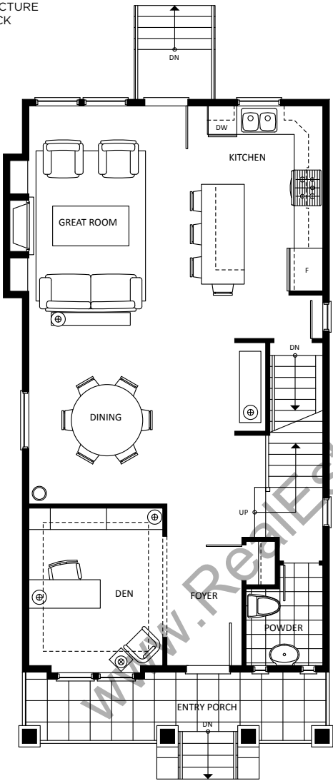
MAIN LEVEL
